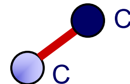
Diamant
