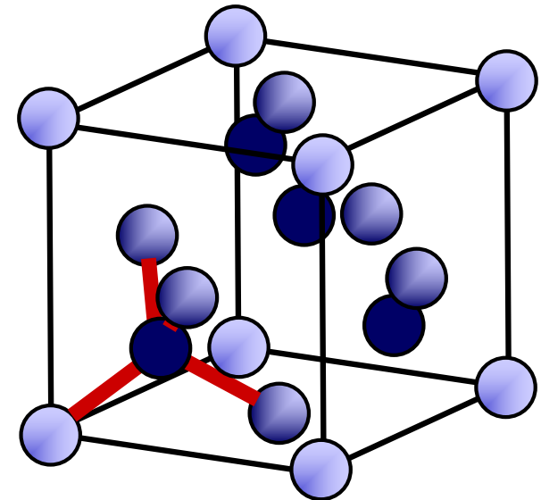
Diamant
